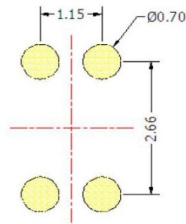
Recommended Solder Pad Layout
