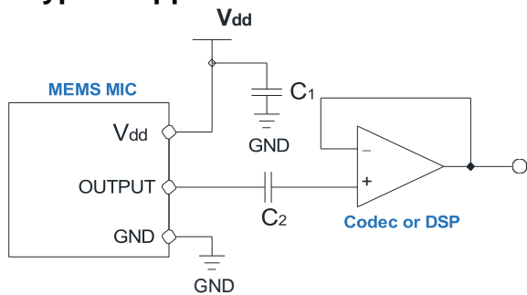
Fig. 10 Single ended input interface circuit
