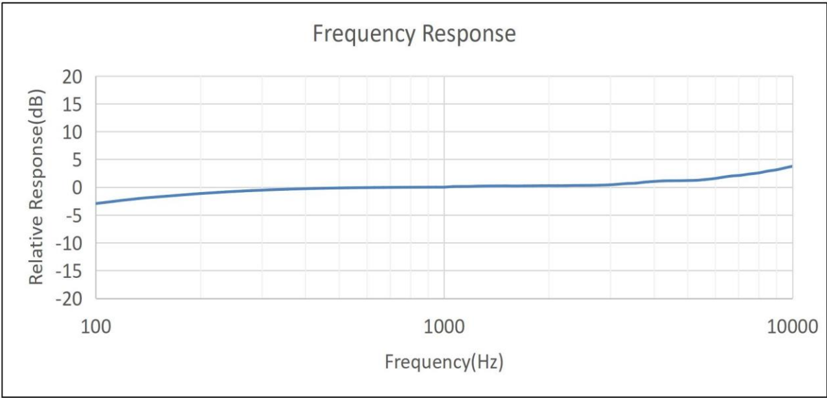
Fig. 2 Frequency response curve normalized to 1kHz
