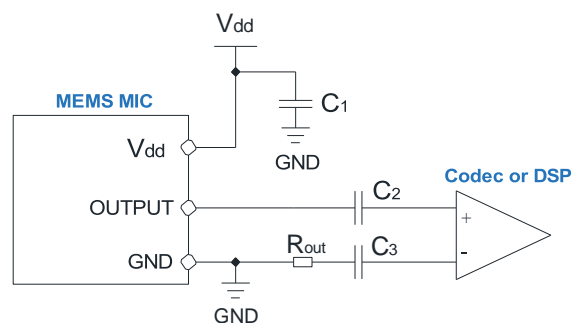
Fig. 11 Differential input interface circuit
