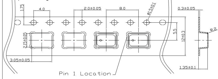
Fig. 9 Packaging
