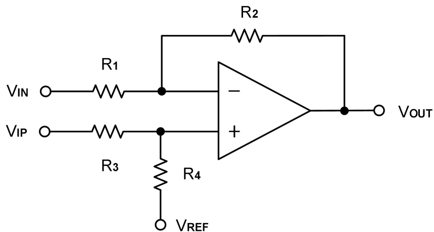
Figure 4. Differential Amplifier
