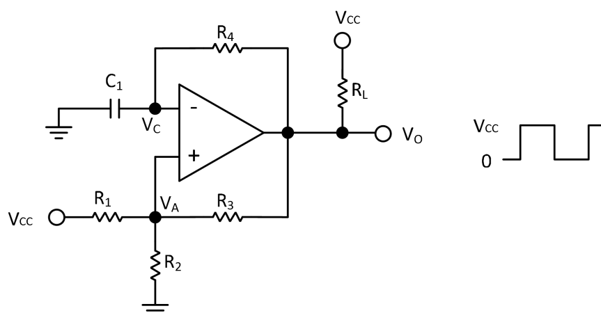
Figure 1. Square-Wave Oscillator
